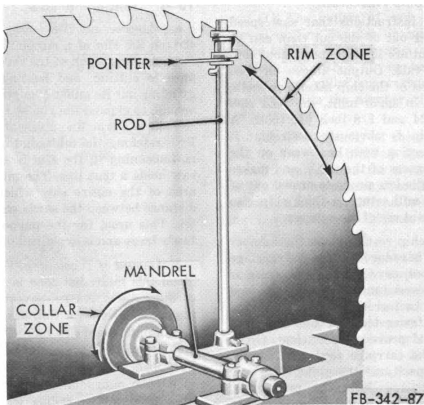
Figure 10-4. Trial mandrel.
